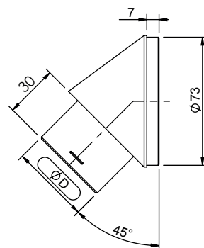
Version sans plaque Version without plate
